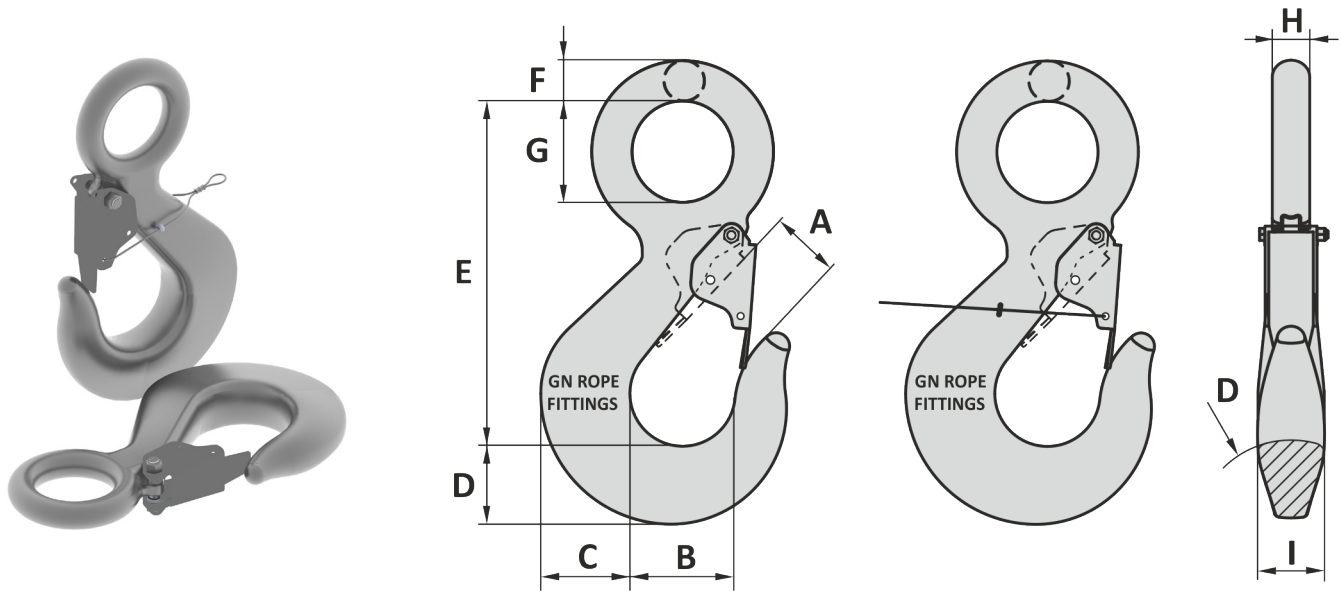
Standard hook with safety latch
